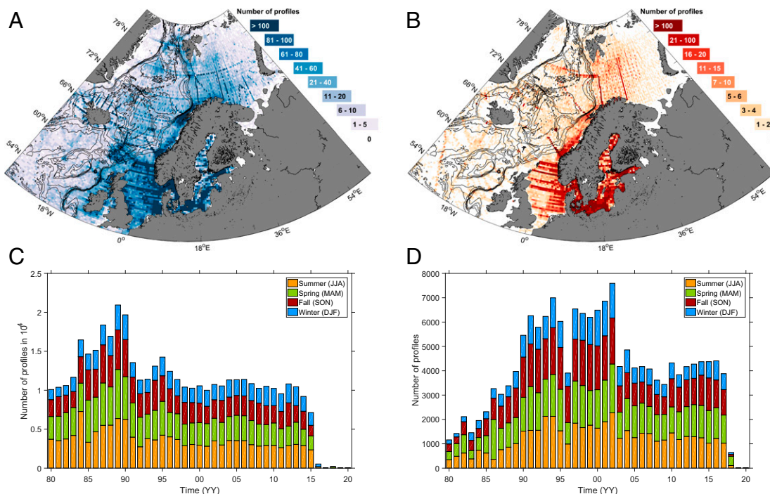
Fig. 1. Data distribution of (A and C) temperature/salinity and (B and D) nutrients/oxygen. (A and B) Total number of vertical profiles per 0.5° longitude × 0.25° latitude bin since 1980. (C and D) Number of vertical profiles per year, color coded by season. Note the different scales. The data were obtained from Unified Database for Arctic and Subarctic Hydrography, ICES, World Ocean Database, the international Argo program, Global Ocean Data Analysis Project version 2, Institute of Marine Research (Norway), Marine and Freshwater Research Institute of Iceland, and the Norwegian Iceland Seas Experiment database. Duplicates between the archives have been discarded. Note the asymmetry in spatial data, with high coverage in the eastern part of the basin where current change is least and vice versa. There is a considerable seasonal bias in data available from the seas neighboring the Nordic countries, with highest density for spring and summer, a feature prone to impact our understanding of past as well as future changes. JJA, June, July, August; MAM, March, April, May; SON, September, October, November; DJF, December, January, February.
